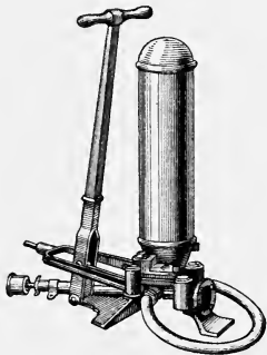
FIG. 46—LARGE HAND PUMP
